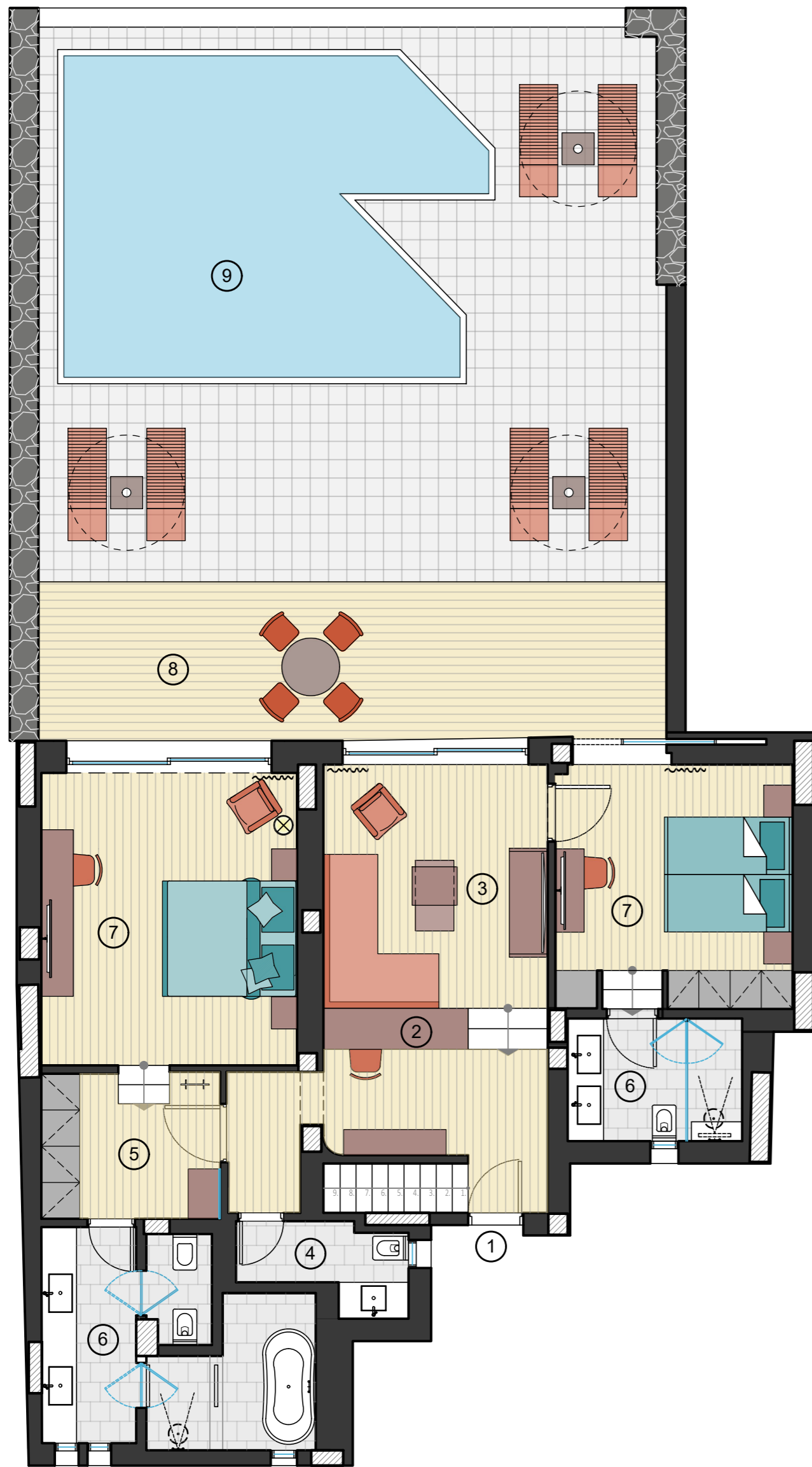
GROUND FLOOR
